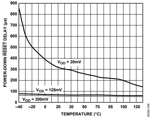
Figure 8. Power-Down \overline{RESET} Delay vs. Temperature (ADM81xL/M)
